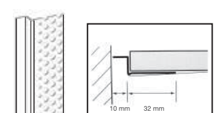
PN 307: Shadowline Stopping Angle (3000 mm) * *MTO
